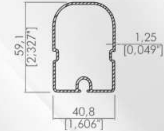
40,8x59,1 İnce Korniş 40,8x59,1 Fabric Support Profile
