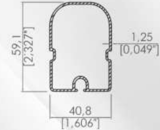
40,8x59,1 İnce Korniş 40,8x59,1 Fabric Support Profile
